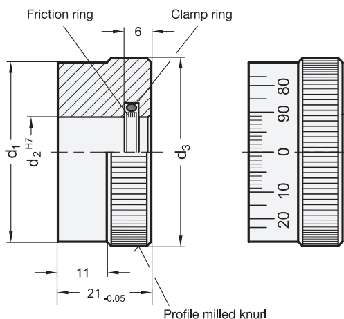
Connection measurements for version with friction ring
